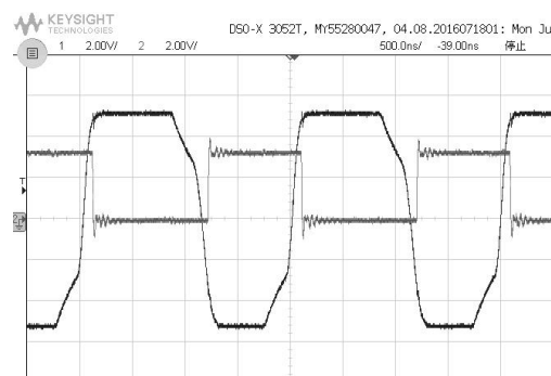
图 2. WS3232F RIN to ROut (3K&amp;250pF load) at 1000kbps waveform
